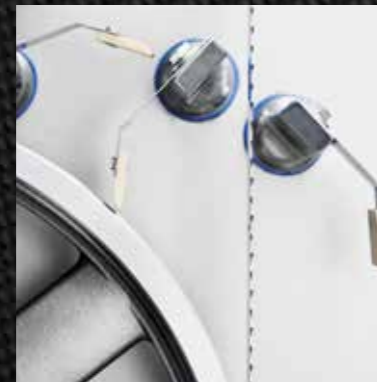
Abklappbare Abstreifer Removable scrapers
